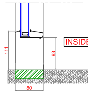
SECTION 'A'-'A' VERTICAL SECTIONS
