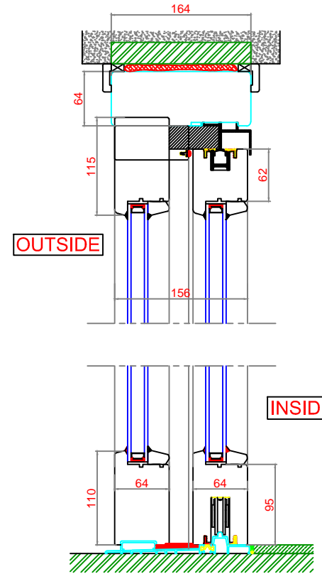
SECTION 'A'-'A' VERTICAL SECTIONS
