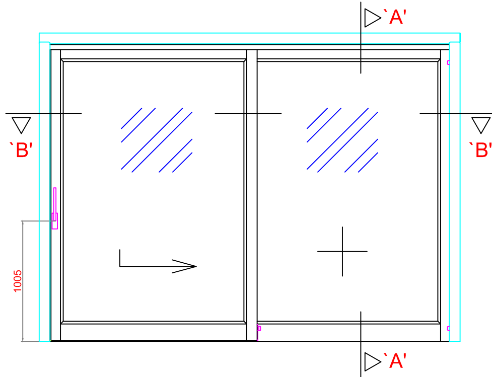
ELEVATION (NTS)
