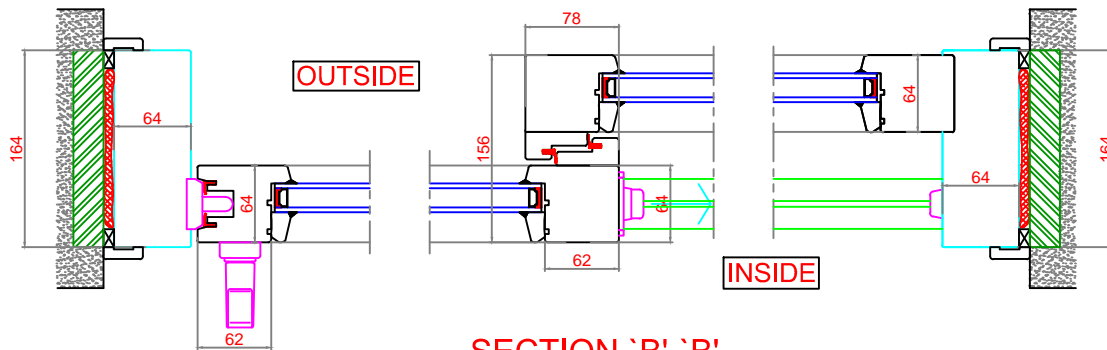
SECTION 'B'-'B' HORIZONTAL SECTION IN PLAN
