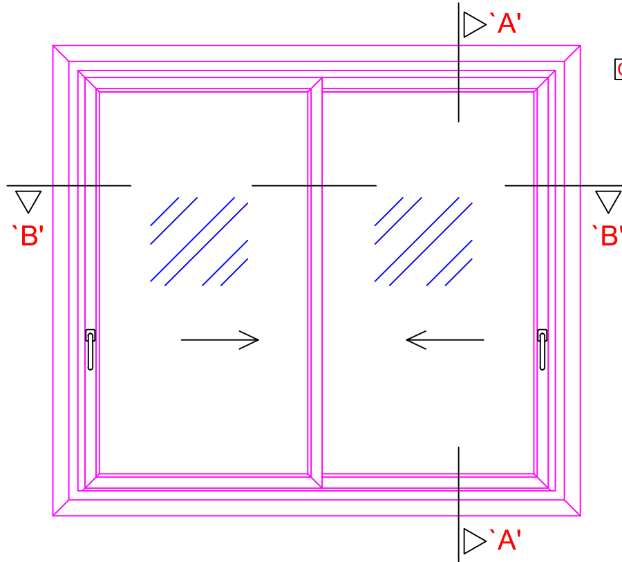
ELEVATION (NTS)
