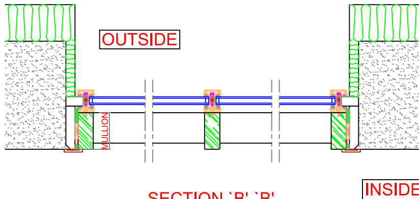
SECTION 'B'-'B' HORIZONTAL SECTION IN PLAN
