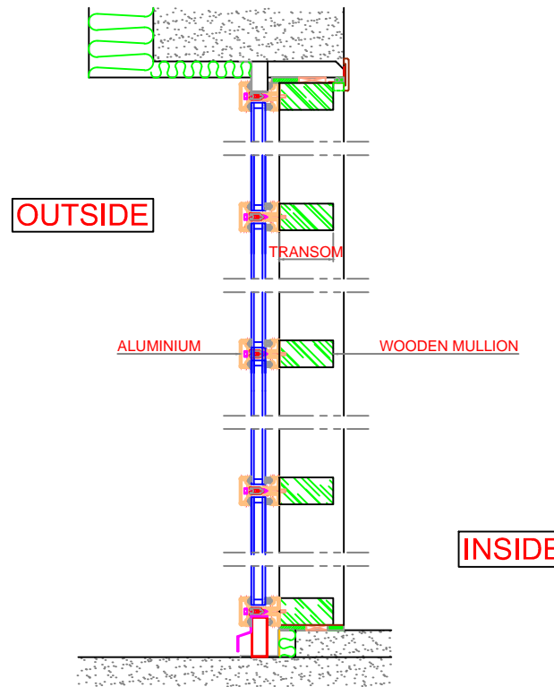
SECTION 'A'-'A' VERTICAL SECTIONS
