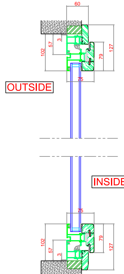
SECTION 'A'-'A' VERTICAL SECTIONS
