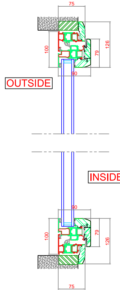
SECTION 'A'-'A' VERTICAL SECTIONS
