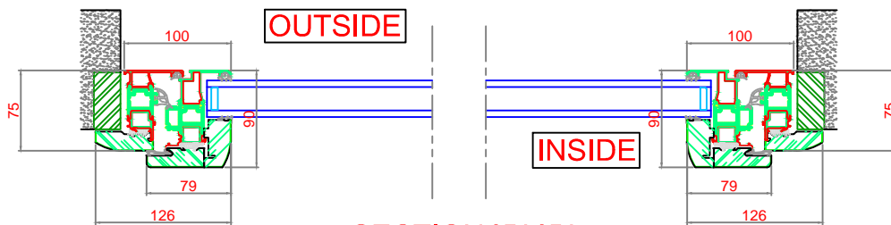
HORIZONTAL SECTION IN PLAN
